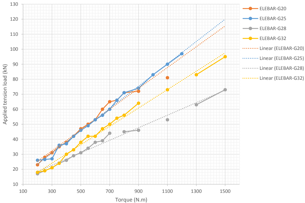
ELEBAR-G torque tension diagram
